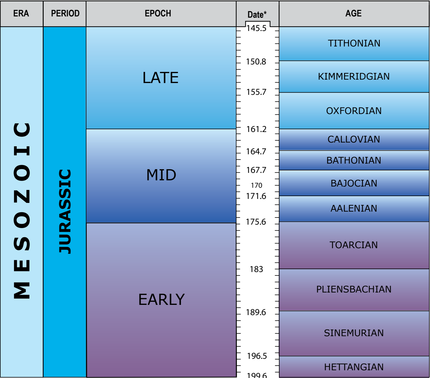
BGS Geological Timechart
