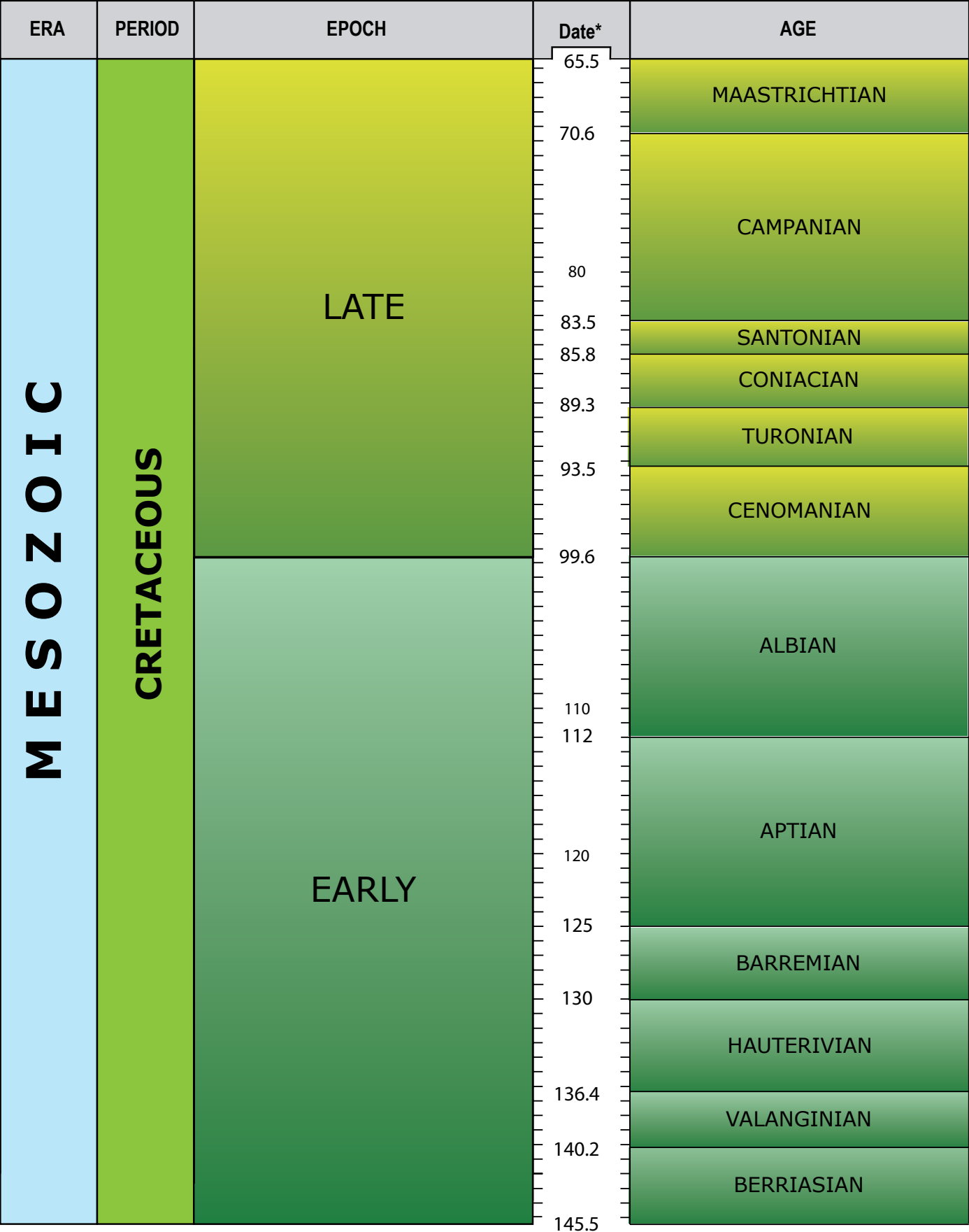
BGS Geological Timechart
