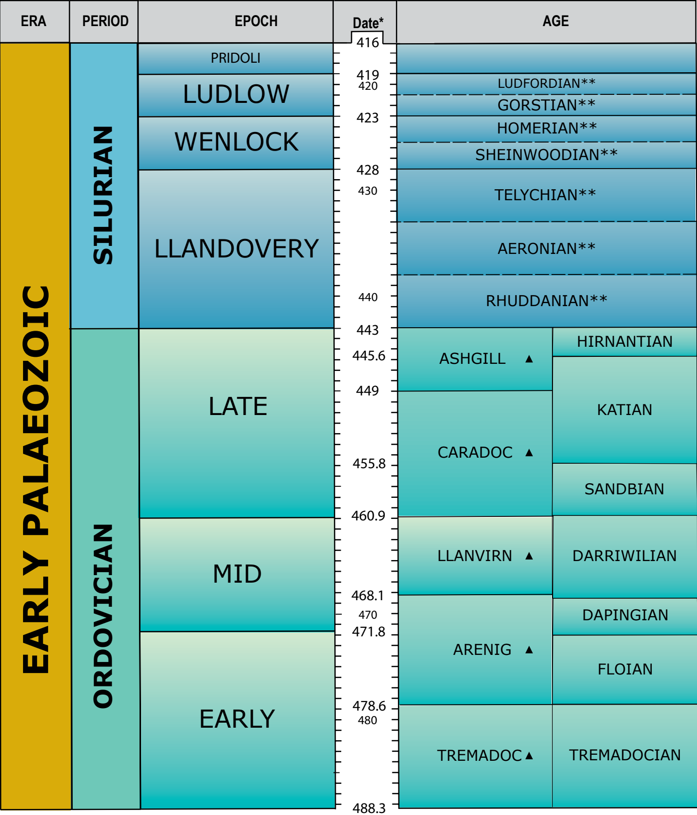
BGS Geological Timechart
