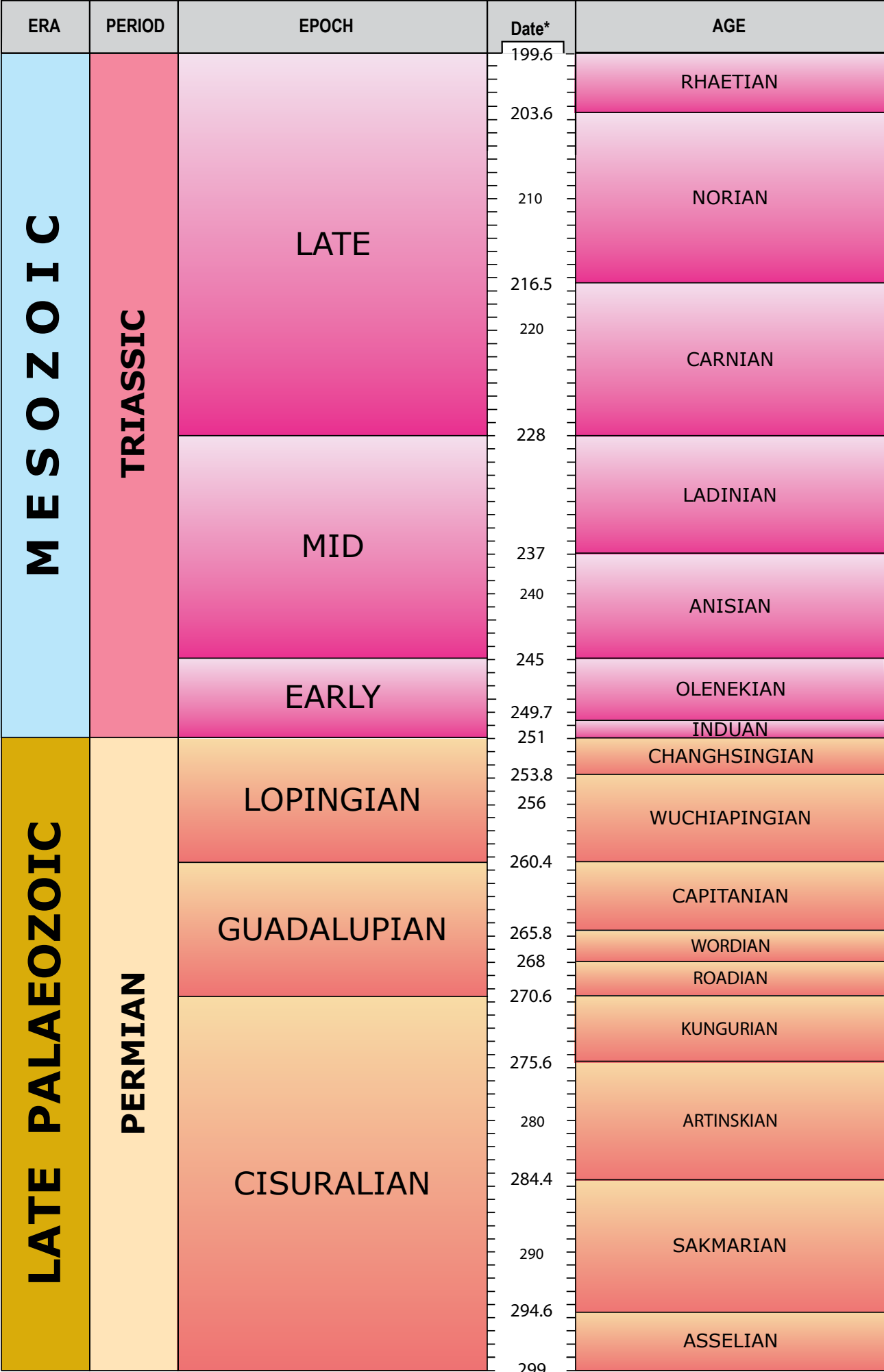
BGS Geological Timechart
