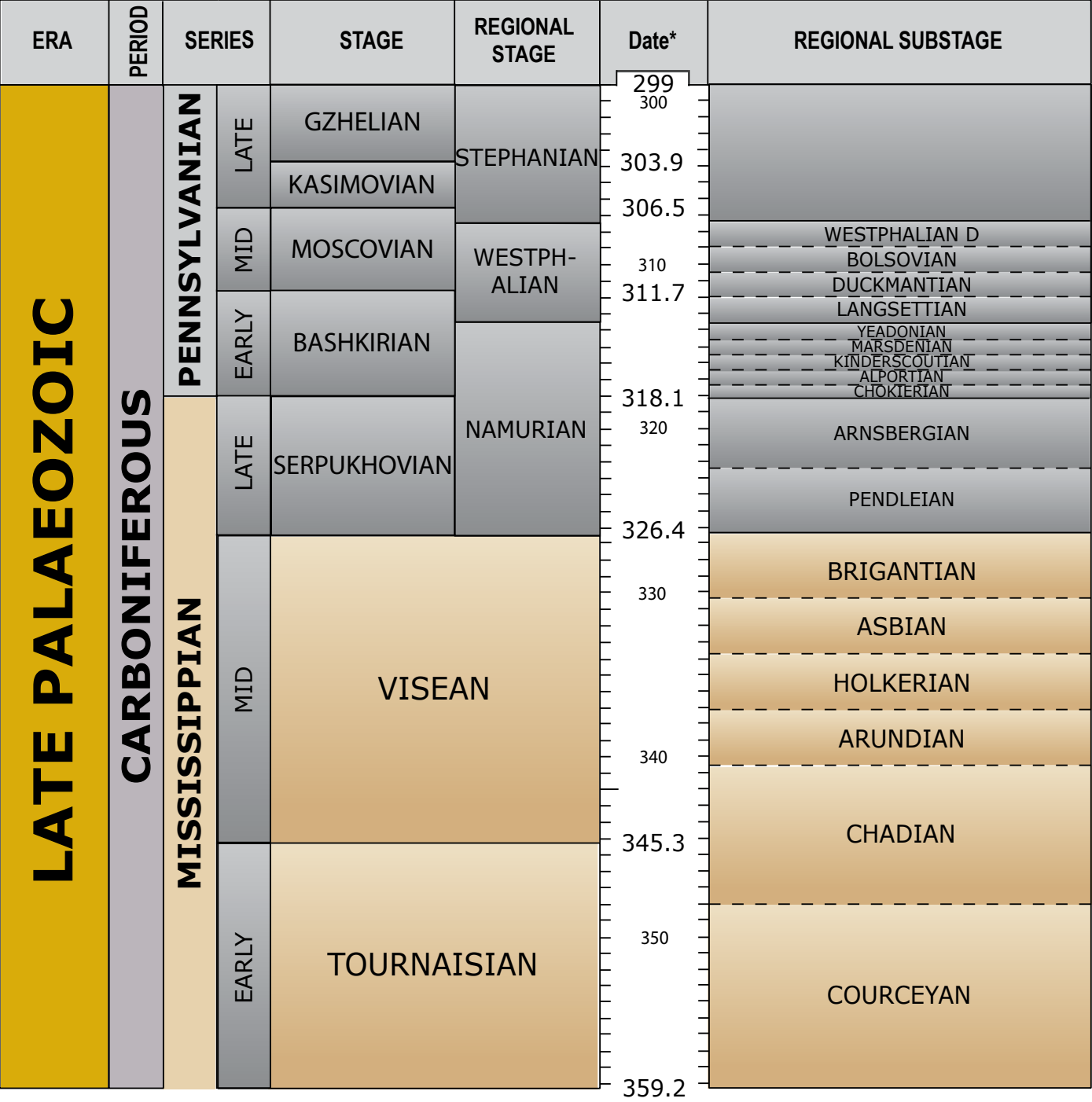
BGS Geological Timechart
